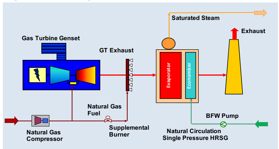
Cogeneration Flow Diagram
