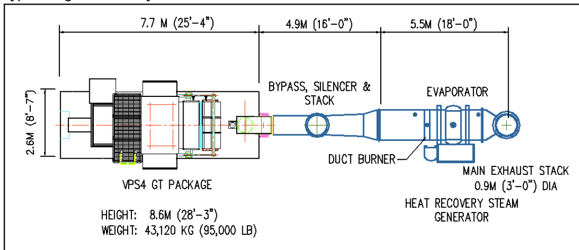
Typical Cogeneration Layout
