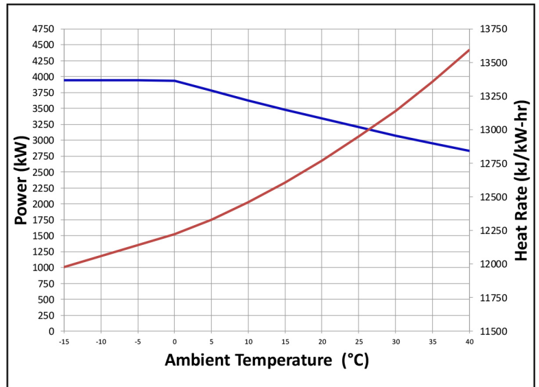
VPS4 - Power & Heat Rate vs Ambient Temperature
