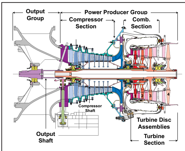
ASE50B Cross-Section
